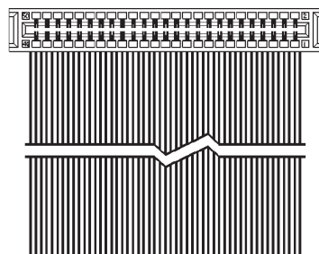
14. IDC 50 Position Socket (Card Edge) Internal cable connector for SCSI and SCSI-2 controllers and peripherals.
