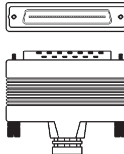
11. .050 Centronics 68M (IBM/PC Workstations) External SCSI connector for SCSI-3 applications with IBM workstations.
