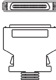
7. .050 CENTRONICS 50M (Mini Centronics) External cable connector for SCSI-2 controllers and peripherals.
