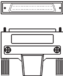
5. .050 50 PIN w/thumbscrews (Hewlett Packard) External SCSI connector for SCSI-2 applications, Hewlett Packard computers and workstations.
